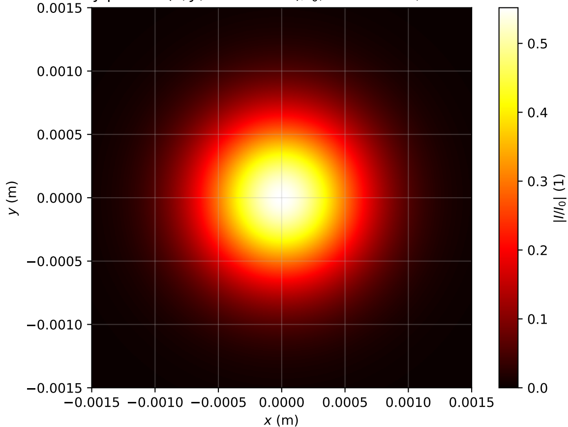
Intensity profile I(x, y, z = 2.388m)/I_0 , P_{in}=0.3P_{cr} , artificial time
